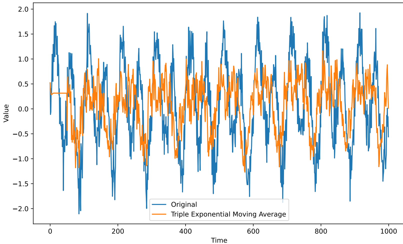
Triple Exponential Moving Average \alpha = 0.6 , \beta = 0.4 , \gamma = 0.2
